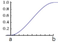
Figure 1: Cubic Hermite Interpolation
