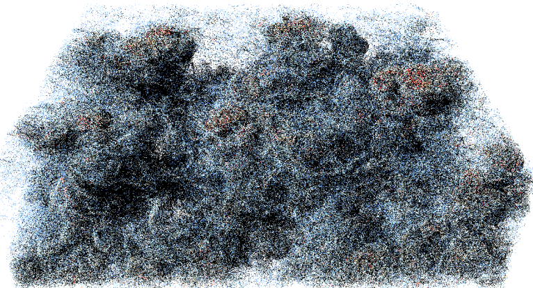
Figure 1: MCFTLE results in ECMWF and CTBL after 1 iteration.
