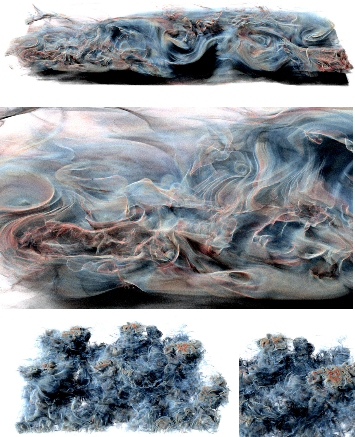
Figure 3: MCFTLE results in ECMWF and CTBL after 200 iterations.
