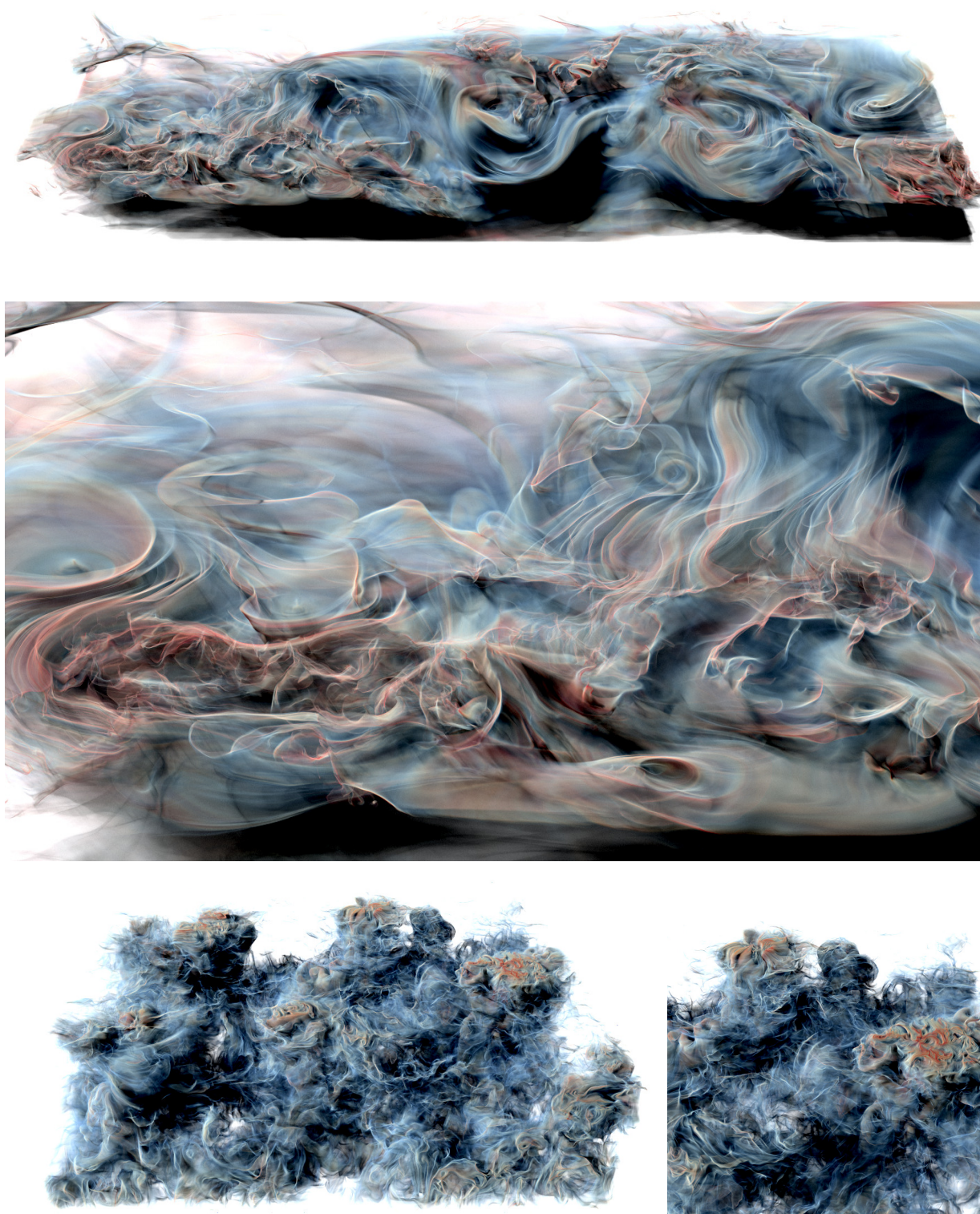
Figure 5: MCFTLE results after 10k (ECMWF), 6.2k (ECWMF CLOSE), 5.2k (CTBL) and 4.4k (CTBL CLOSE) iterations.
