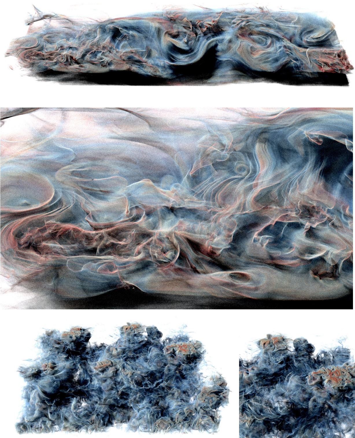
Figure 2: MCFTLE results in ECMWF and CTBL after 100 iterations.
