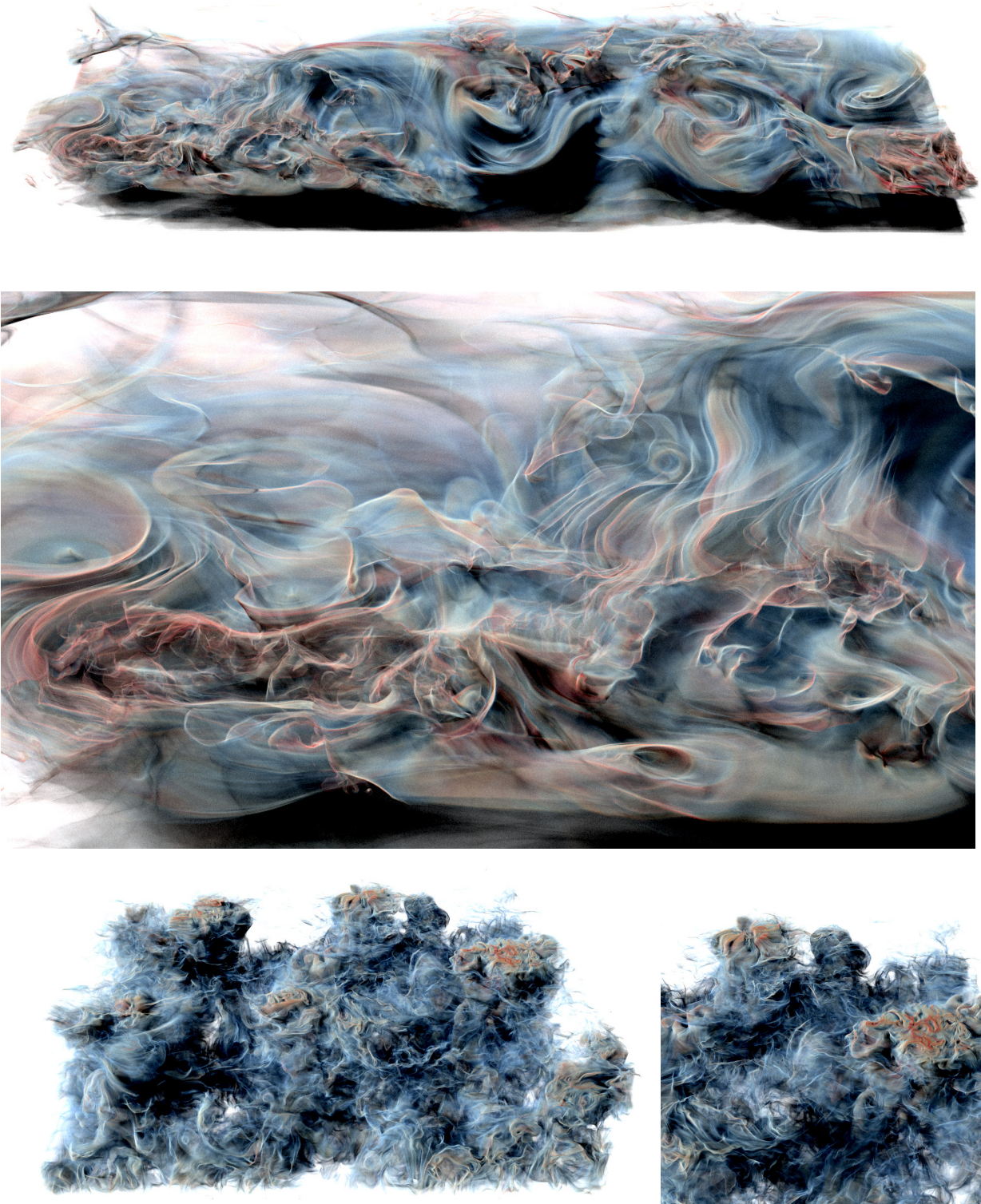
Figure 4: MCFTLE results in ECMWF and CTBL after 1000 iterations.
