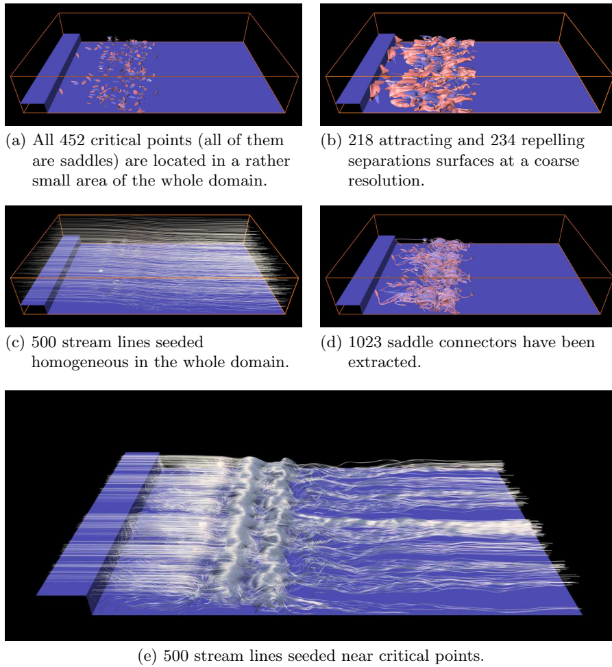
Fig. 5. Flow around a backward-facing step.
