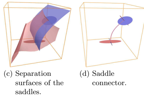
Fig. 8. Critical points and definition of saddle connectors.
