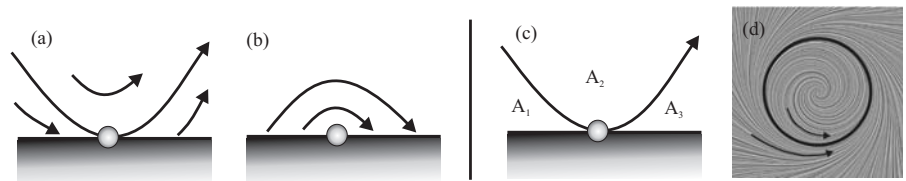
Fig. 4. (a) inbound boundary switch point; (b) outbound boundary switch point; (c) separatrix from inbound boundary switch points divides the domain into 3 sectors A_1, A_2, A_3 ; (d) an isolated closed stream line divides the domain into 2 sectors.
