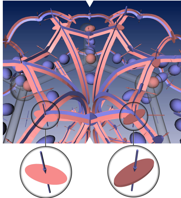
Figure 4: Topological skeleton of the benzene data set showing saddle connectors and critical points. Left: Outflow/inflow planes of the saddle points depicted with flat ellipses. Right: Our enhanced design using elliptic cylinders.
