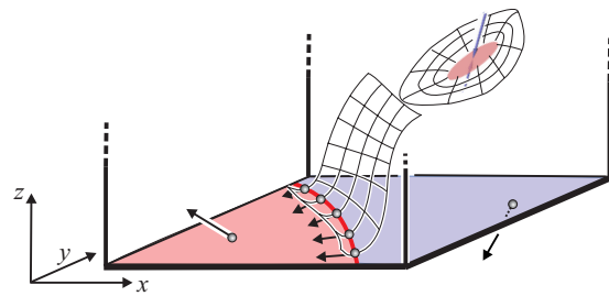
Figure 12: Finding the intersection of two separation surfaces – one comes from a saddle, while the other one comes from a boundary switch curve; shown is the situation short before an intersection is found; in the next integration step an intersection point \mathbf{p}_1 is found which defines the boundary switch connector.
