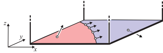
Figure 5: Boundary plane z = z_{min} consisting of an inflow area (blue), an outflow area (red), and their separating boundary switch curve; shown are 4 vectors of \mathbf{v} on the boundary switch curve, and one each in the inflow and outflow area.
